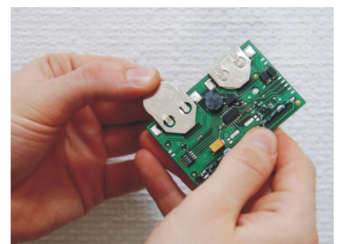
Step 4: Inserting of batteries in the alarm transmitter and done!
